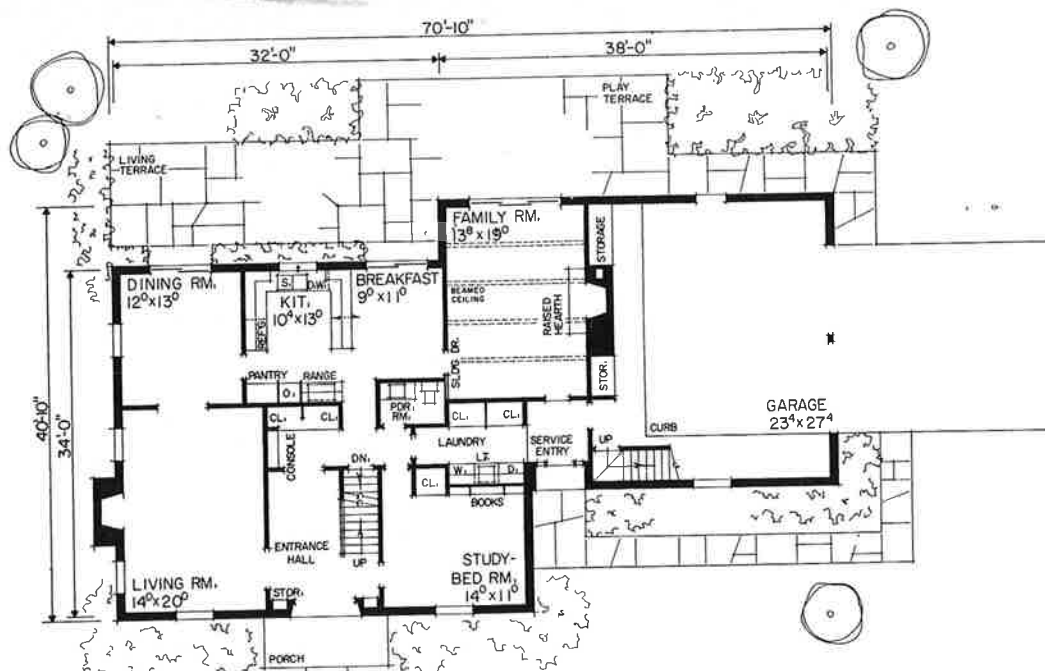
Design 11934 1,622 Sq. Ft. - First Floor; 2,002 Sq. Ft. - Second Floor; 51,758 Cu. Ft.
