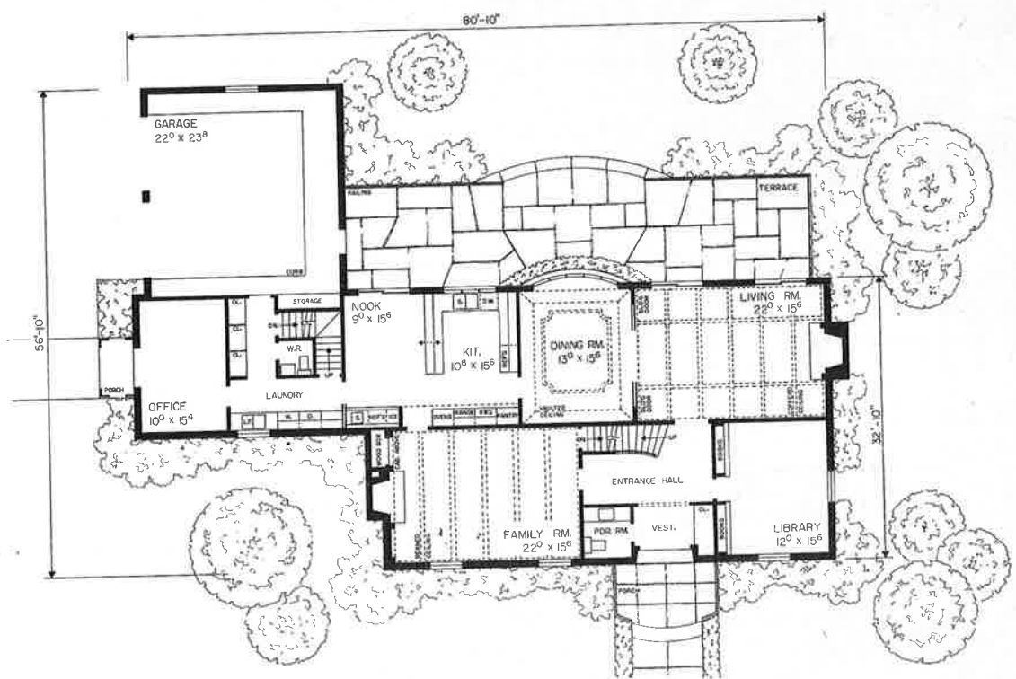
Design 11839 2,204 Sq. Ft. - First Floor; 1,486 Sq. Ft. - Second Floor; 330 Sq. Ft. - Maid's Area; 55,683 Cu. Ft.
