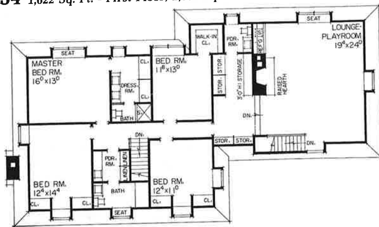
Design 11934 1,622 Sq. Ft. - First Floor; 2,002 Sq. Ft. - Second Floor; 51,758 Cu. Ft.
