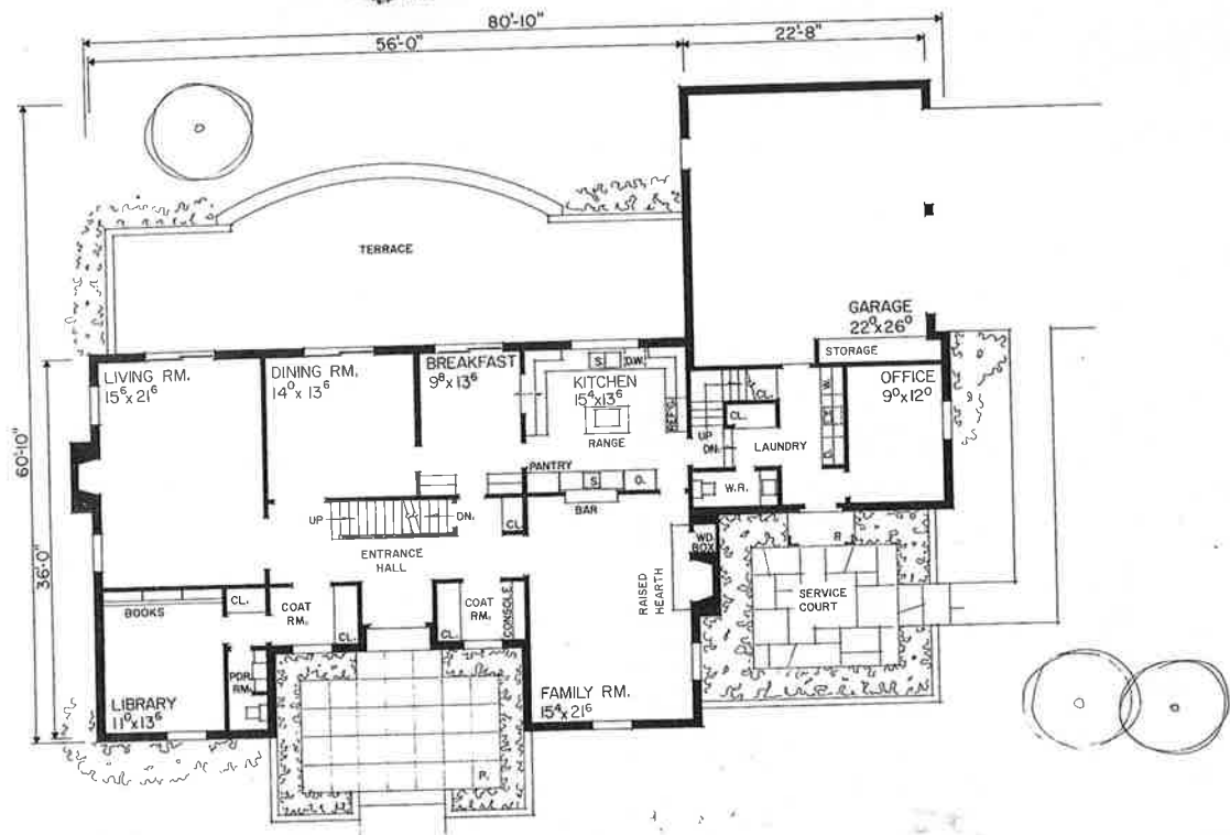
Design 11826 2,230 Sq. Ft. - First Floor; 1,576 Sq. Ft. - Second Floor; 308 Sq. Ft. - Maid's Area; 52,852 Cu. Ft.
