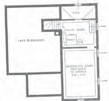
FOUNDATION PLAN
