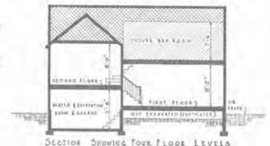
SECTION SHOWING FOUR FLOOR LEVELS
