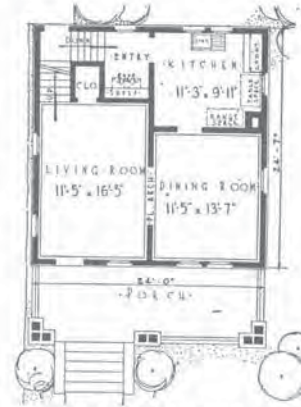
FIRST FLOOR 3315-A
