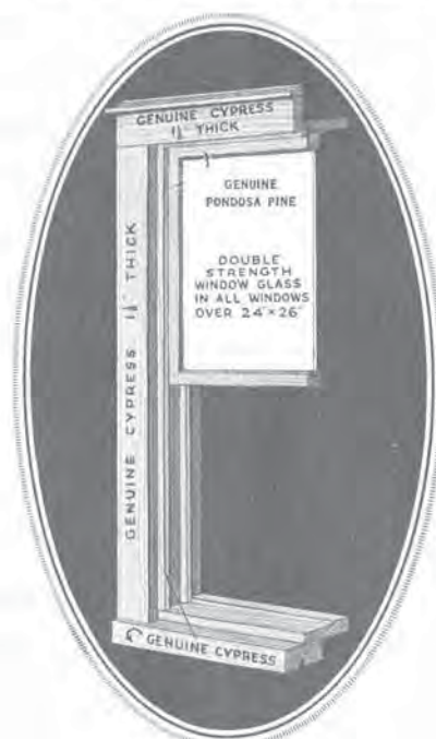
Above section shows all members of frame to be genuine cypress and window sash of Clear Ponderosa Pine
