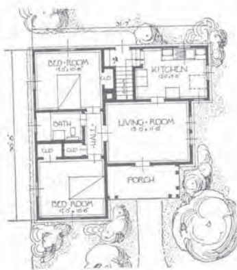
FLOOR PLAN
