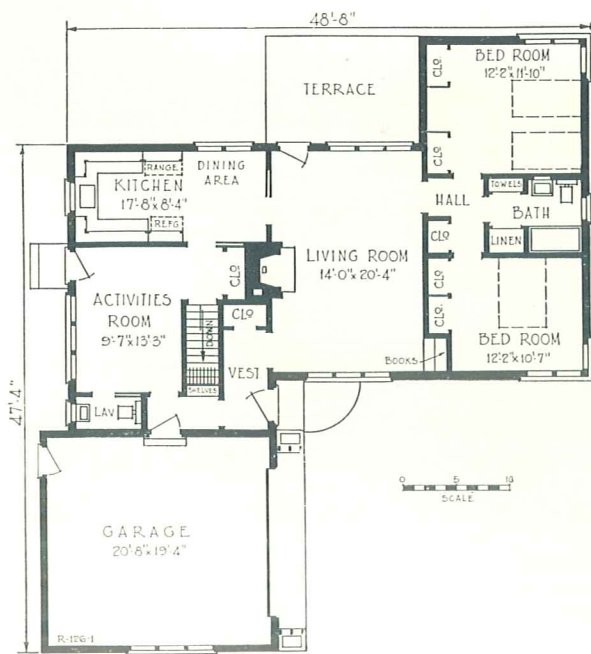
PLAN 1—WITH BASEMENT
