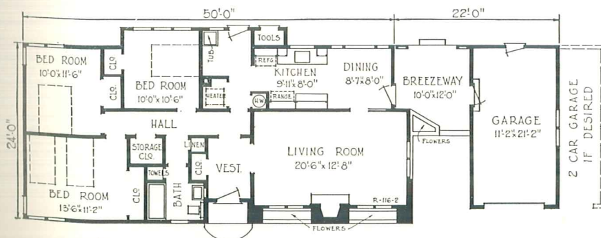
PLAN 2—WITHOUT BASEMENT
