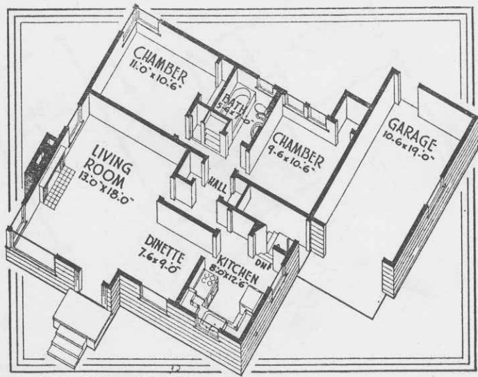
FLOOR PLAN No 4723-C SIZE - 30.0' x 30.0'
