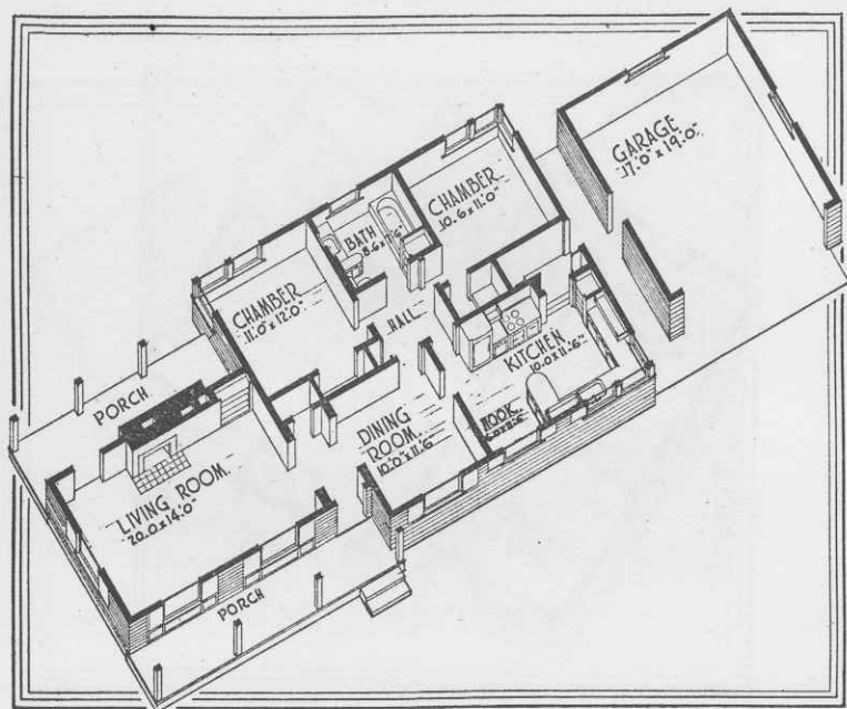
FLOOR PLAN No 5024. SIZE (INCLUDING GARAGE) 34.6 x 27.6"
