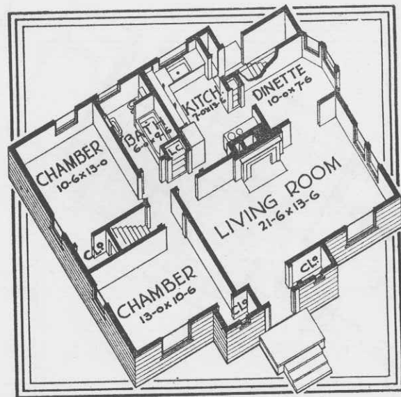
FLOOR PLAN No 4856
