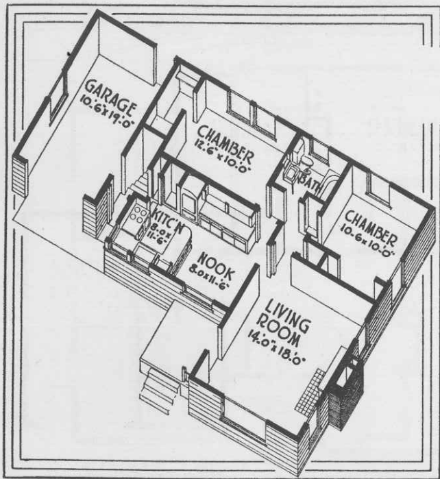
FLOOR PLAN No 4260 SIZE - 46.0' x 32.0'
