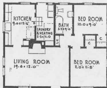
FLOOR PLAN 32.0' x 26.0' PLAN No 4131
