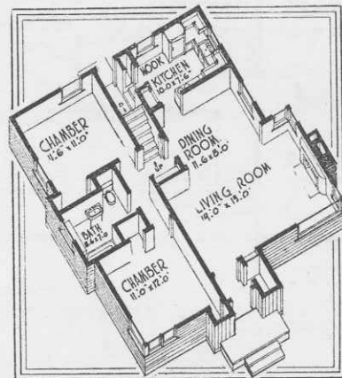
FLOOR PLAN No 5280 SIZE 31.6 x 34.0
