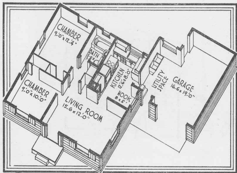
FLOOR PLAN No 4430 SIZE: 41.0" x 36.6"
