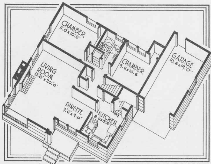
FLOOR PLAN, NO 4723_F SIZE - 41.0 x 32.0 (INCLUDING GARAGE)
