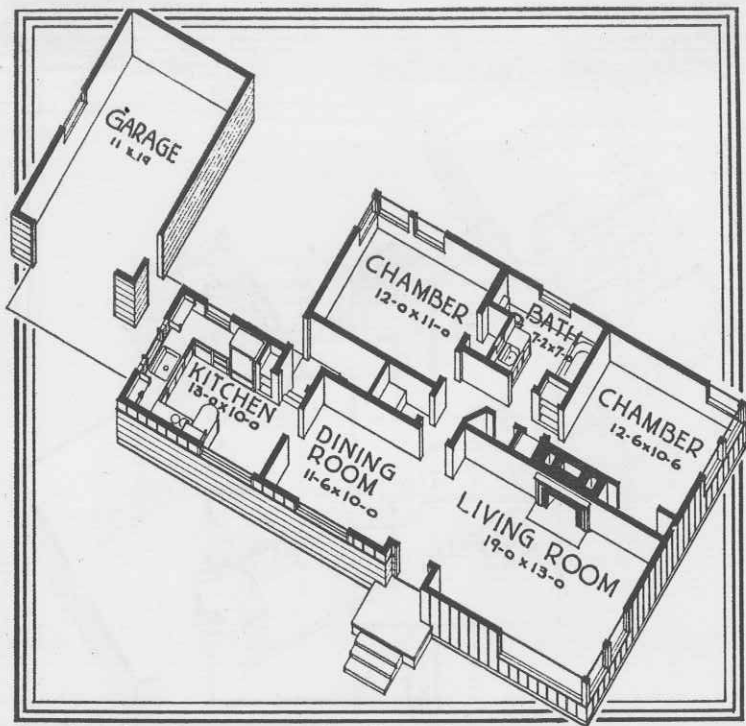
FLOOR PLAN No 5372
