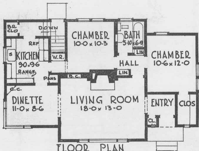
FLOOR PLAN 41-6 x 26-0 PLAN No 5090 AREA 979 SQ. FT.
