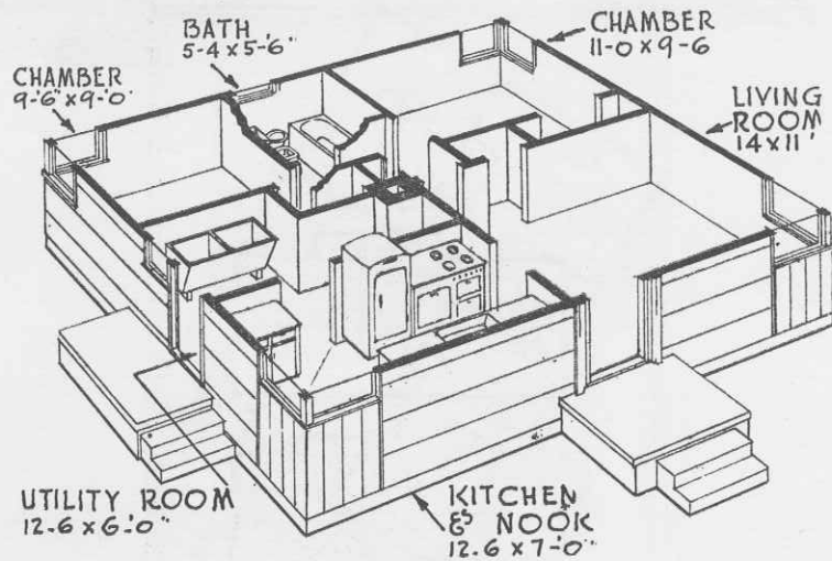
FIRST FLOOR PLAN No 4013 SIZE - 28.0' x 24.0' AREA 672 SQ. FT.
