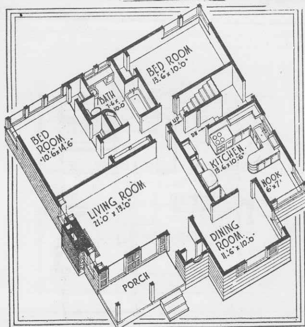
FLOOR PLAN NO 5722 SIZE 36'-0" x 35'-0"
