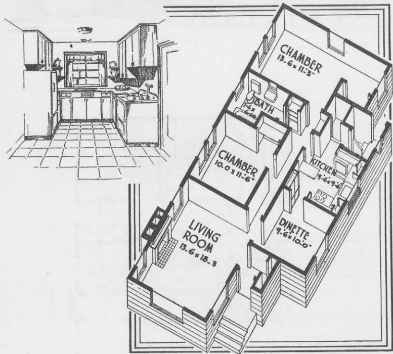
FLOOR PLAN No 5101 SIZE - 24'-6" x 50'-6"
