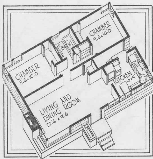
FLOOR PLAN No 4823 SIZE - 34'-0" x 24'-0"
