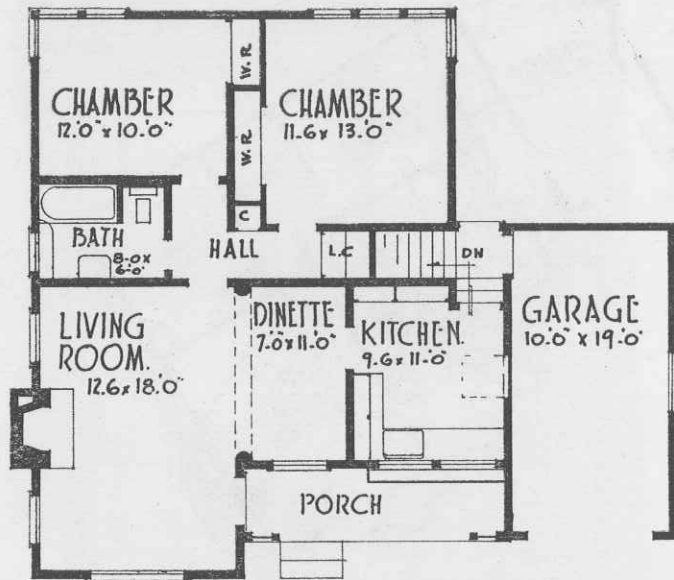
FIRST FLOOR PLAN NO 4188
