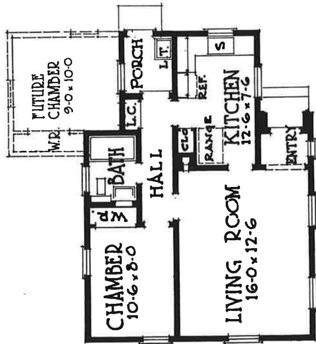
FLOOR PLAN No 3005 30-0 x 22-0
