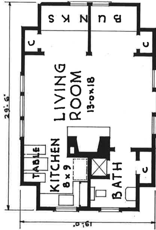
PLAN NO. 106 AREA 532 SQ. FT.
