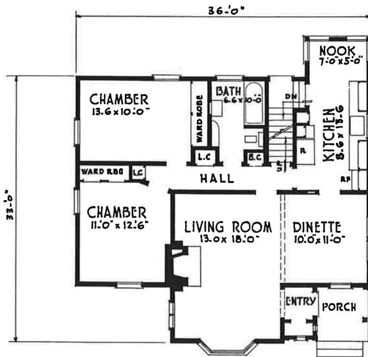
FLOOR PLAN No 5190 AREA 1100 SQ. FT.
