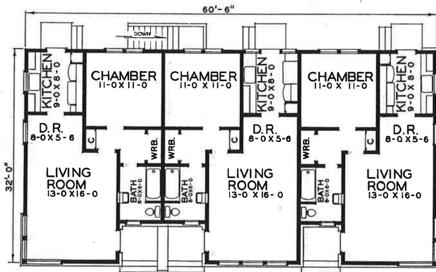
FLOOR PLAN NO. M-3001 AREA 1825 SQ. FT.
