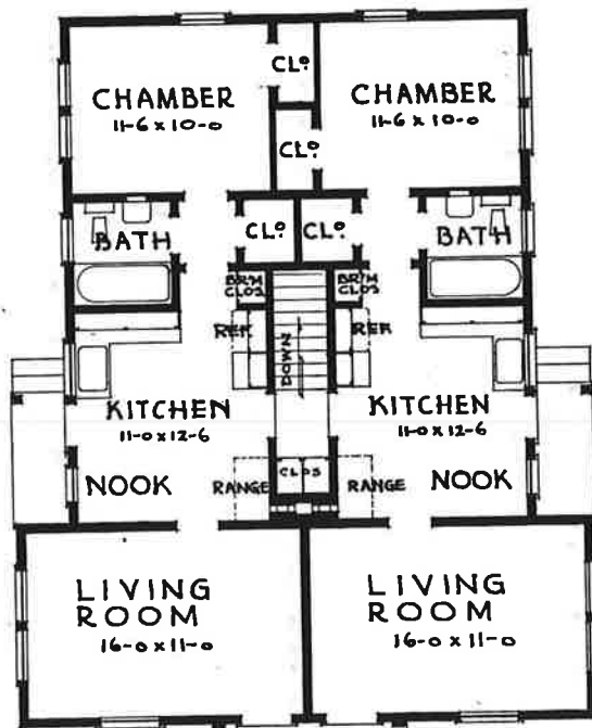
FLOOR PLAN PLAN Nº D-3101 SIZE 33'-6" x 42'-0" AREA 1206 SQ.FT.
