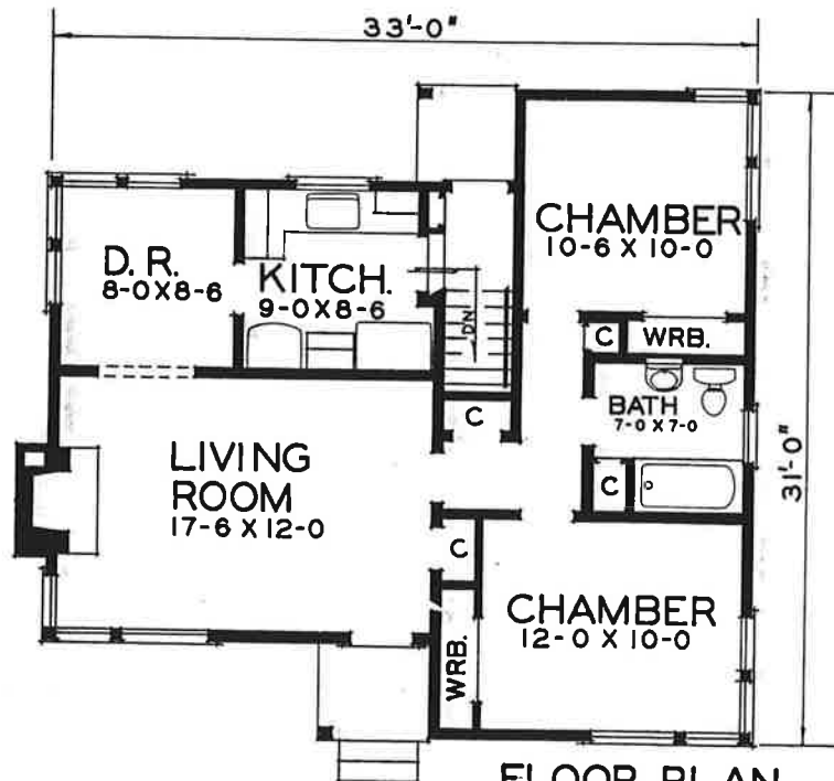
FLOOR PLAN NO 4916 AREA 845 SQ. FT.
