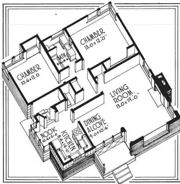
FLOOR PLAN NO 5726 SIZE 32.0 x 35.0
