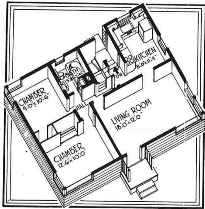
FLOOR PLAN No 4248-B AREA 780 SQ.FT.
