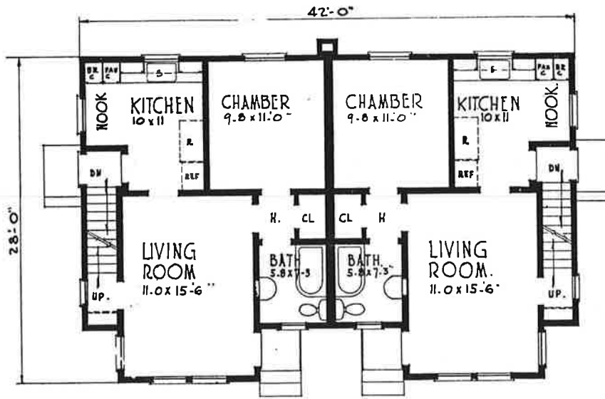
Size 42'-0" x 28'-0" — Area 1095 sq. ft.
