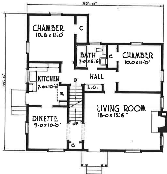
FLOOR PLAN PLAN N9 5030 32.0" x 26.0"
