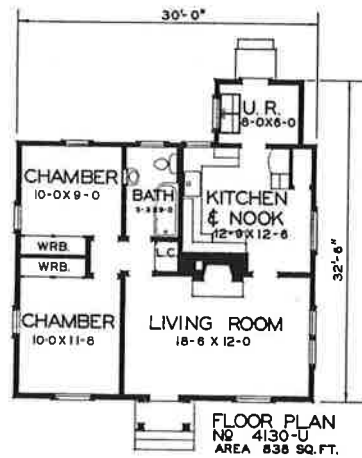
ALTERNATE PLAN With utility room and no basement
