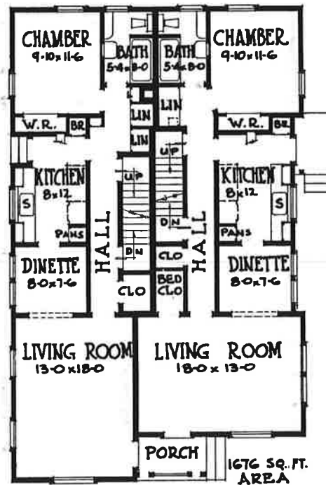
FLOOR PLAN 33-0 x 53-6 PLAN NO. D-500
