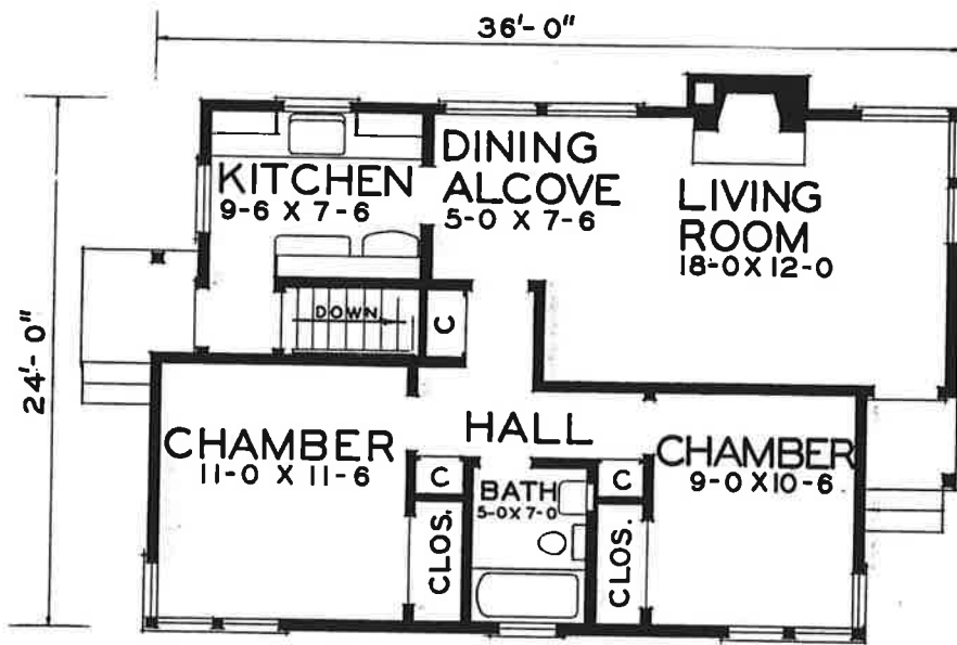
FLOOR PLAN NO. 5551 AREA 797 SQ. FT.
