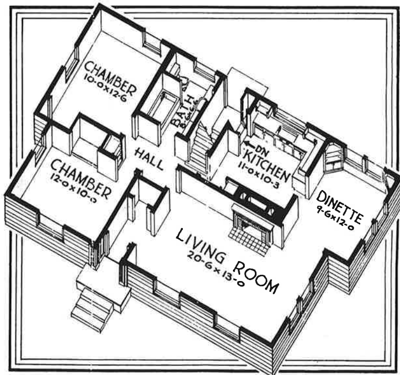
FLOOR PLAN No 5156 SIZE 43'-0" x 26'-6"
