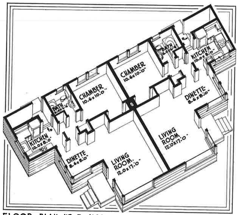
FLOOR PLAN NO D_4160 SIZE - 36'-8" x 31'-0"
