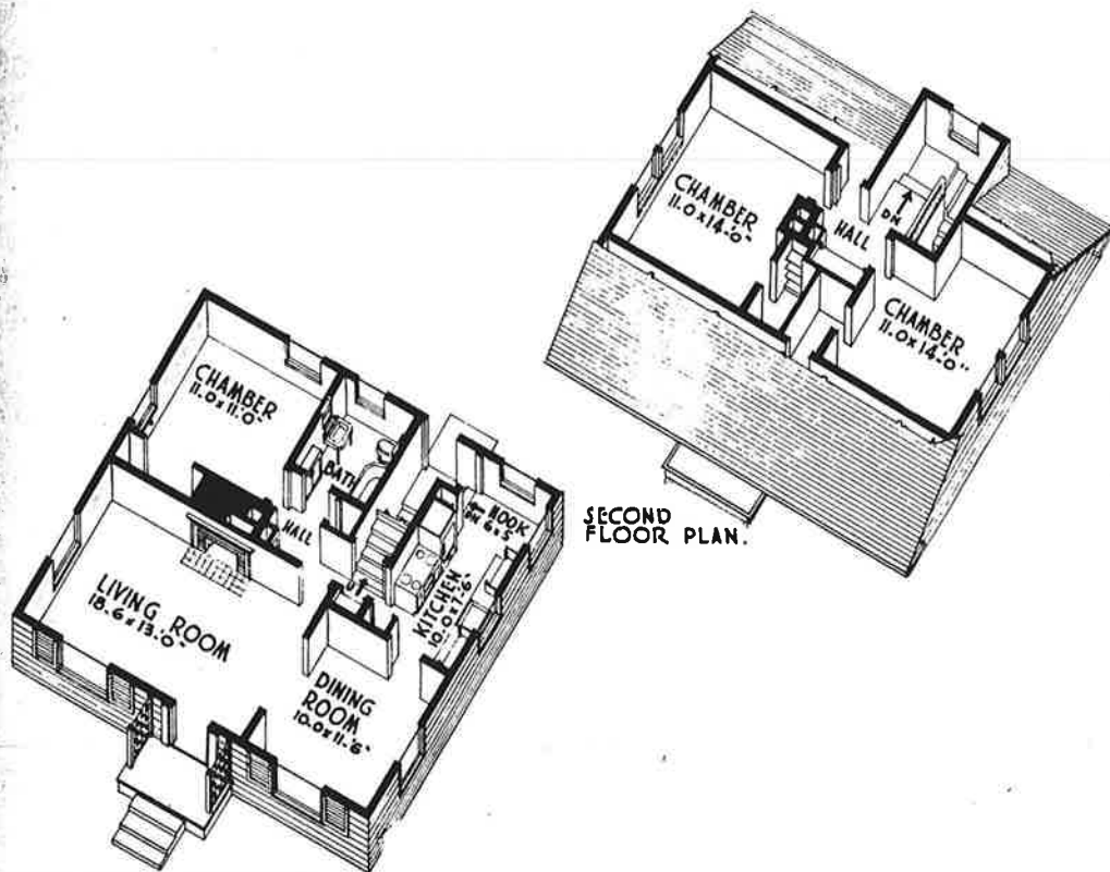
FIRST FLOOR PLAN 6863. SIZE 30.0' x 28.0'
