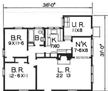
FIRST FLOOR PLAN NO. 4456-U AREA - 976 SQ. FT.
