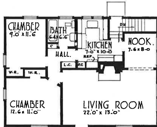
FIRST FLOOR PLAN NO. 4456 SIZE - 36.0 x 26.0 AREA - 936 SQ. FT.
