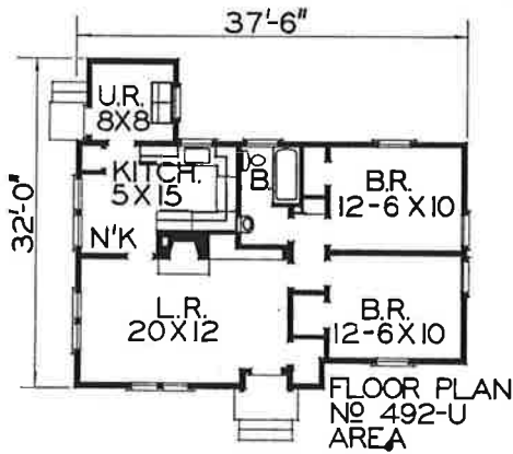
ALTERNATE PLAN With utility room and no basement
